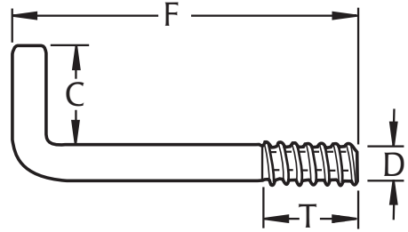
Hook Bolt (Right Angle Bend)
