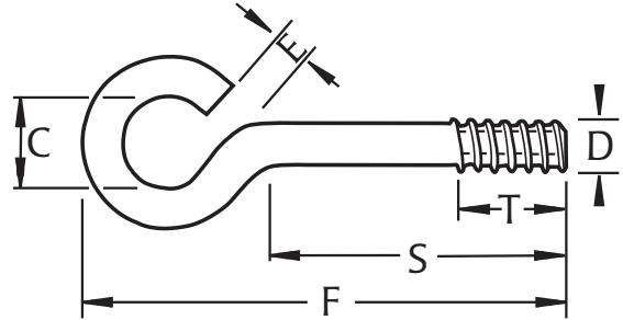
Eye Bolt (Open)
